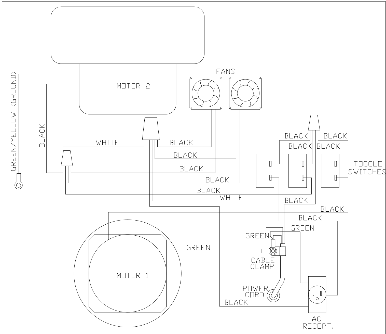
WIRING DIAGRAM MODEL 1200
